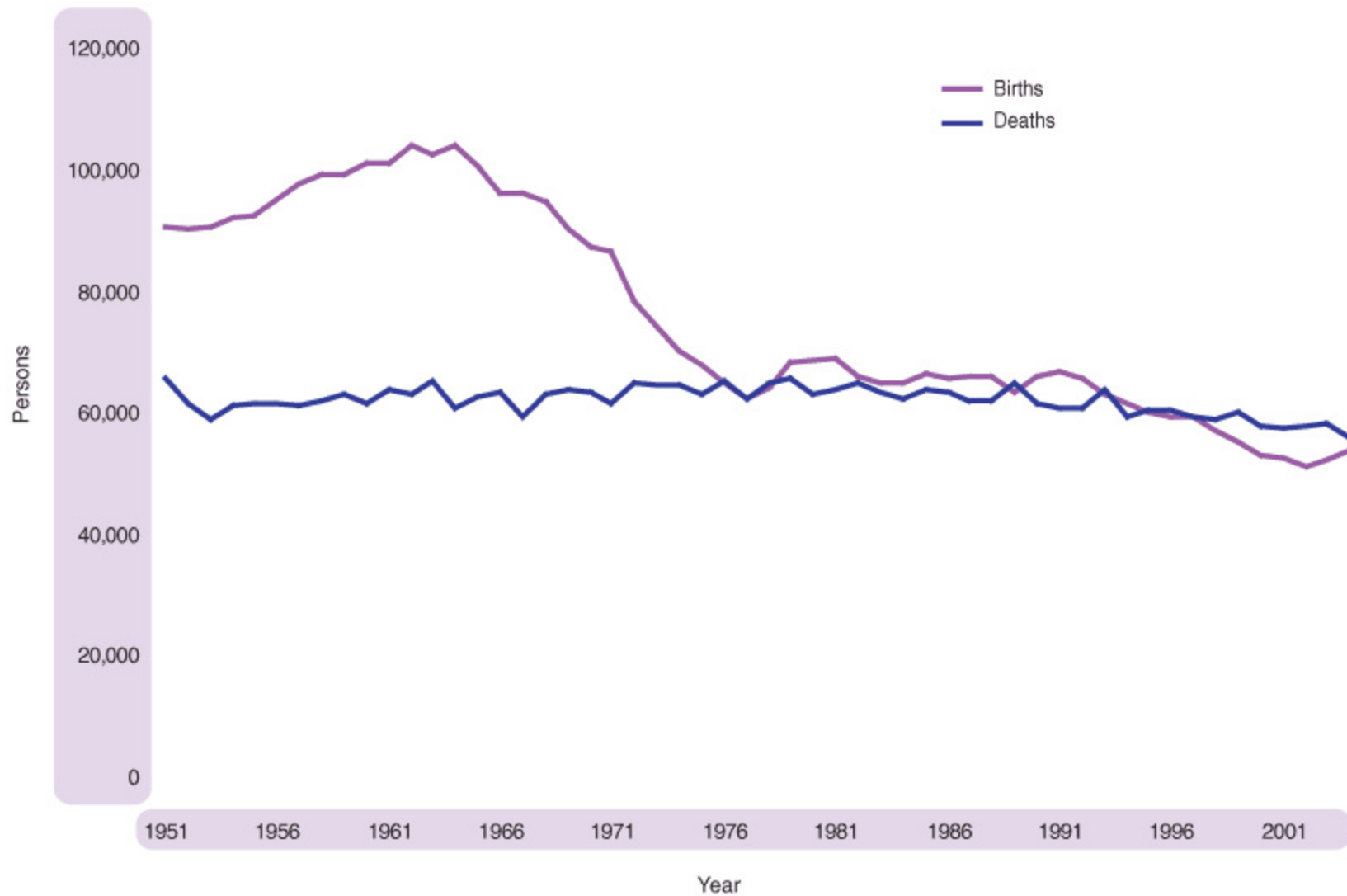
Figure 1.10 Births and deaths, Scotland, 1951-2004
