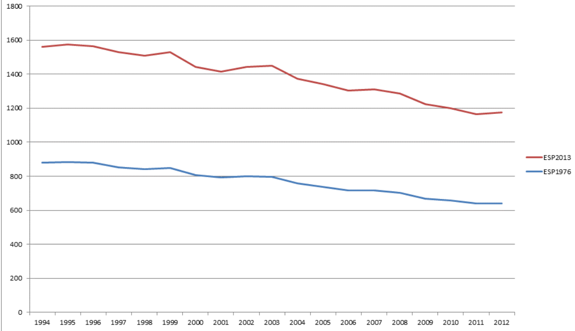
Chart 1: All-age, All-cause Age-standardised mortality rates using the 1976 ESP and 2013 ESP
