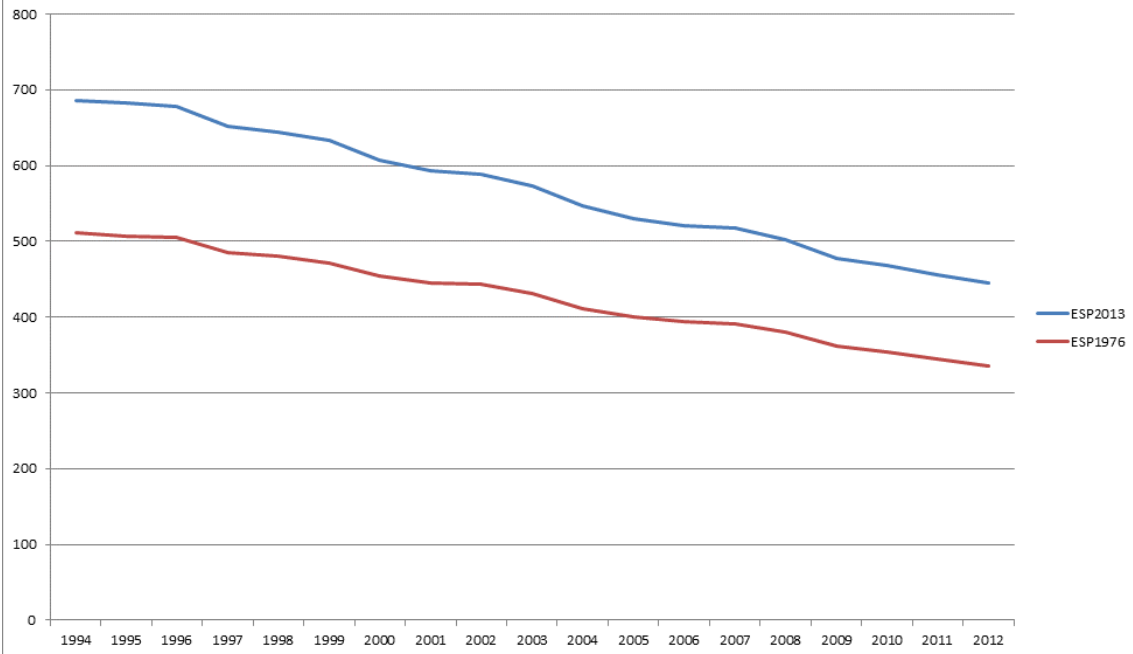
Chart 2: Under 75, All-cause Age-standardised mortality rates using the 1976 ESP and 2013 ESP
