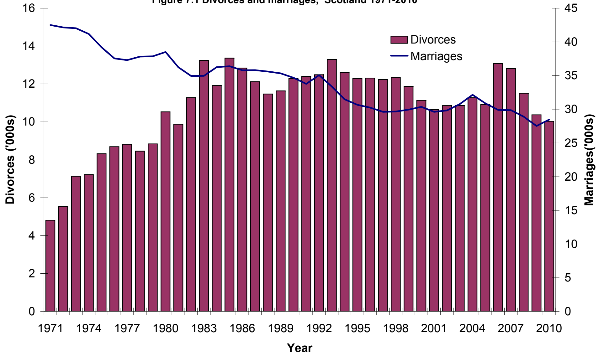
Figure 7.1 Divorces and marriages, Scotland 1971-2010
