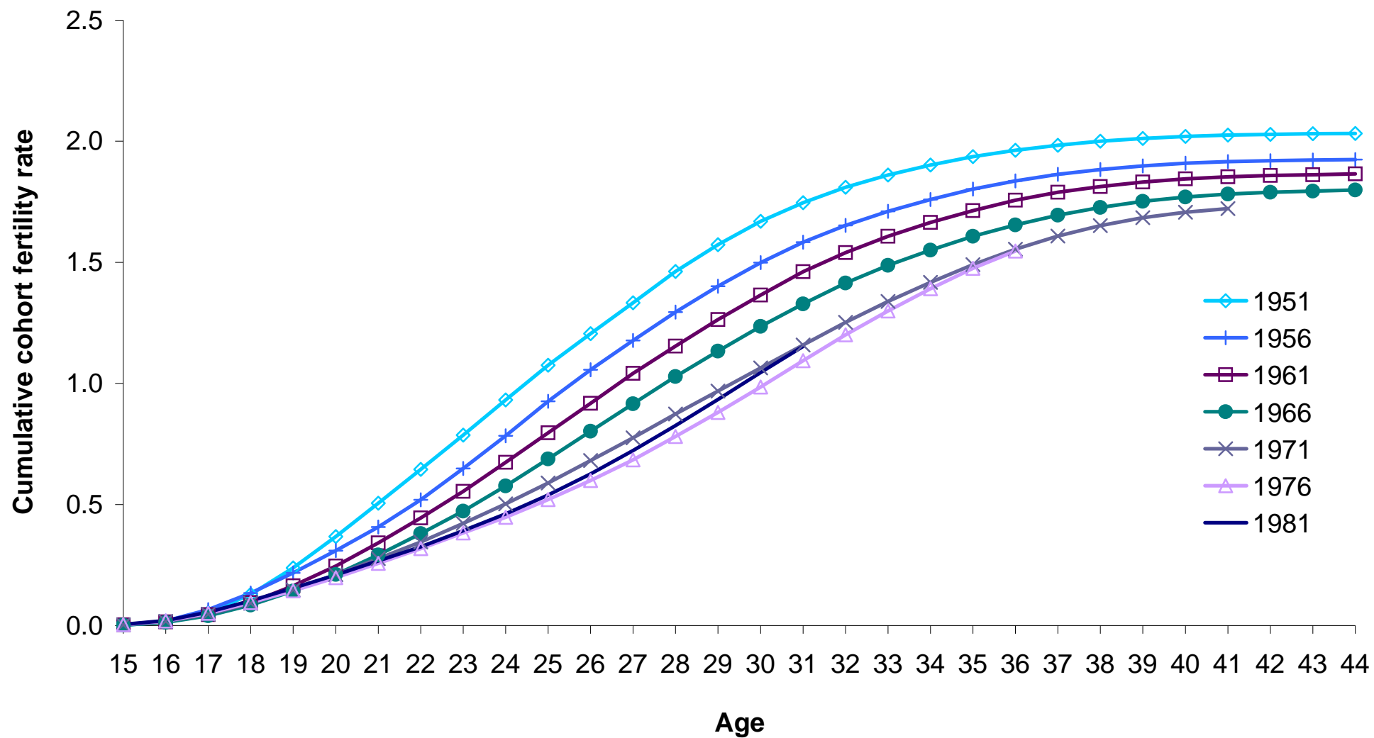
Figure 2.6: Cumulative cohort fertility rate for selected birth cohorts, Scotland
