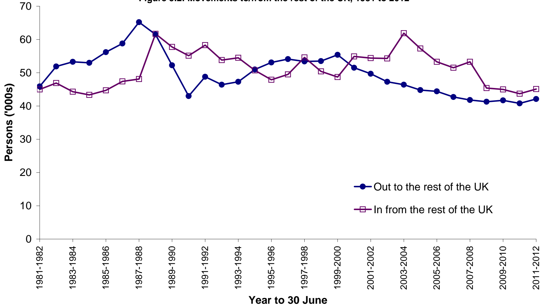
Figure 5.2: Movements to/from the rest of the UK, 1981 to 2012
