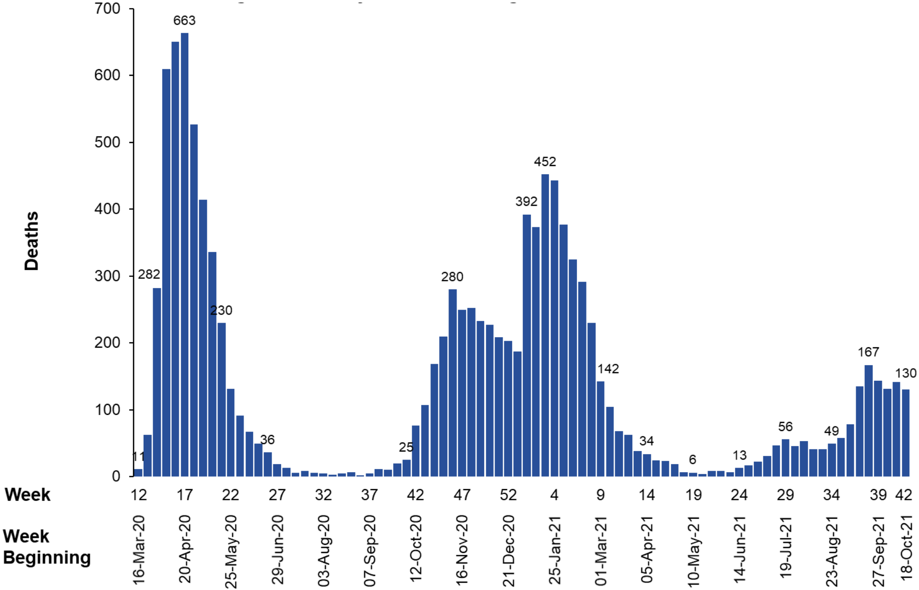
Figure 1: Weekly deaths involving COVID-19 in Scotland, week 12 2020 to week 42 2021
