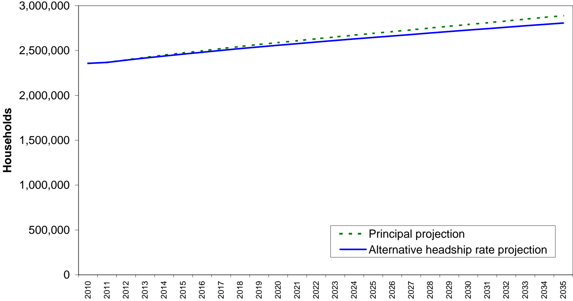
Figure 10: Principal and alternative headship variant household projections for Scotland, 2010 - 2035
