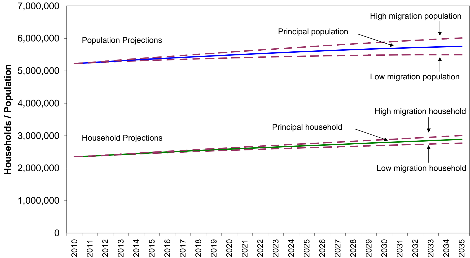
Figure 8: Principal, low and high migration variants, 2010-based population and household projections for Scotland
