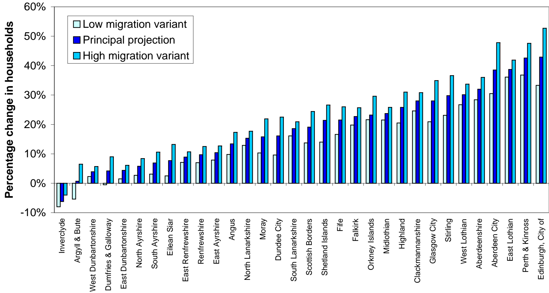
Figure 9: Projected percentage change in households, 2010-2035 principal, low and high migration variant projections, by local authority
