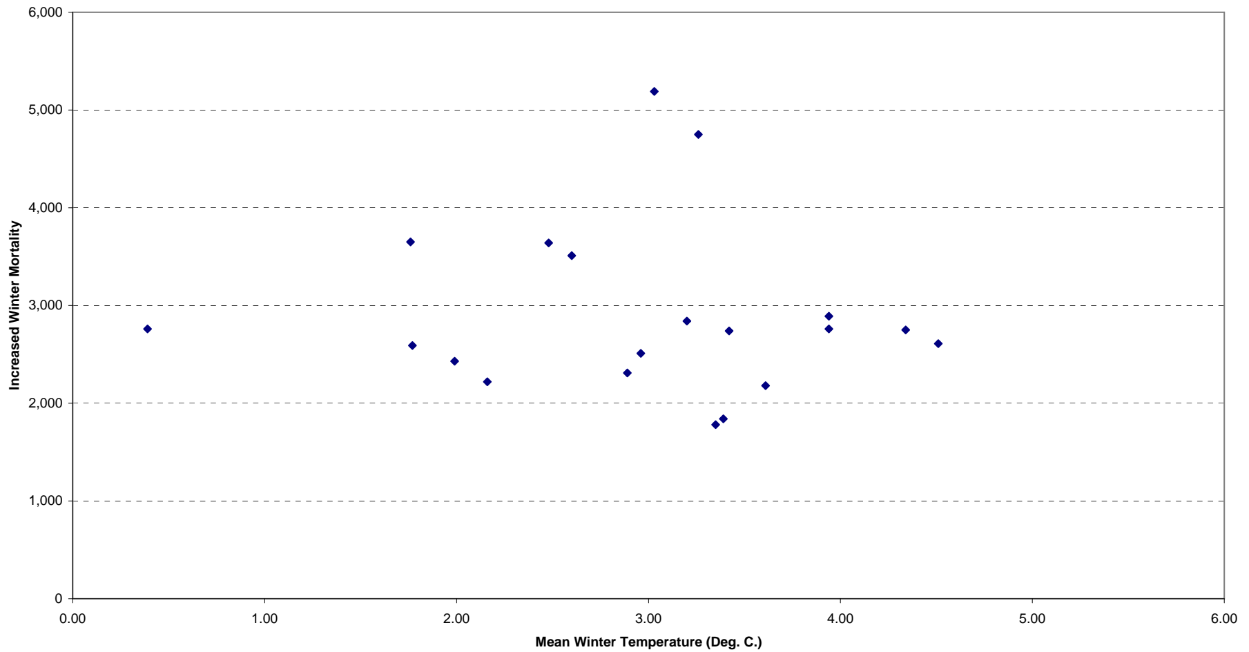
Chart 2 - Increased winter mortality and mean winter temperature, Scotland (b) winter 1990/91 to winter 2009/10
