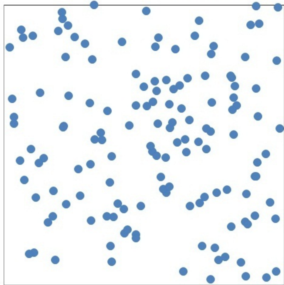
Figure 12: Number of people per square kilometre, Baile a'Mhanaich (Balivanich), Scotland, and Faifley, 2012
