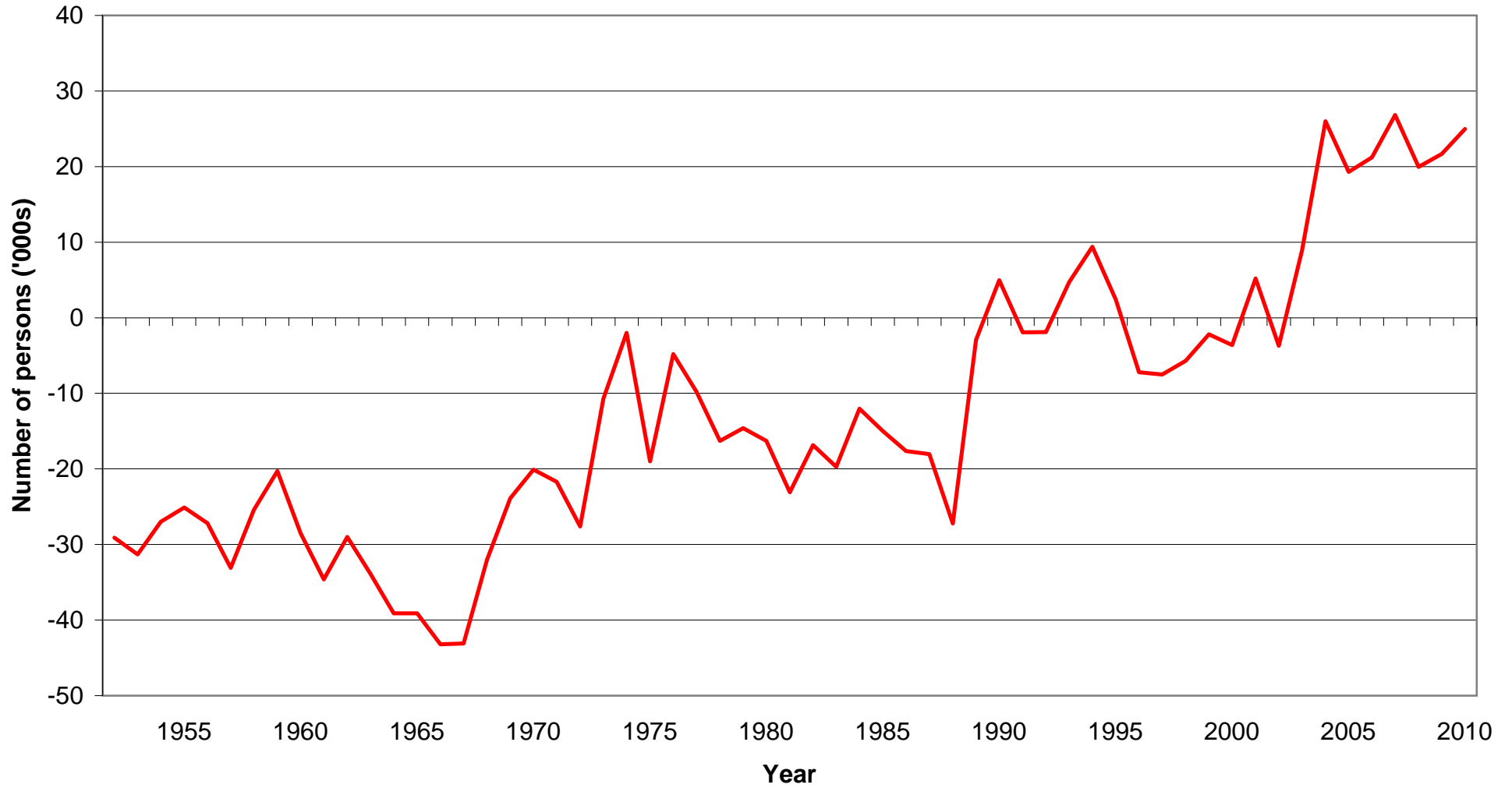
Figure C1 Estimated net migration, Scotland, 1951-2010
