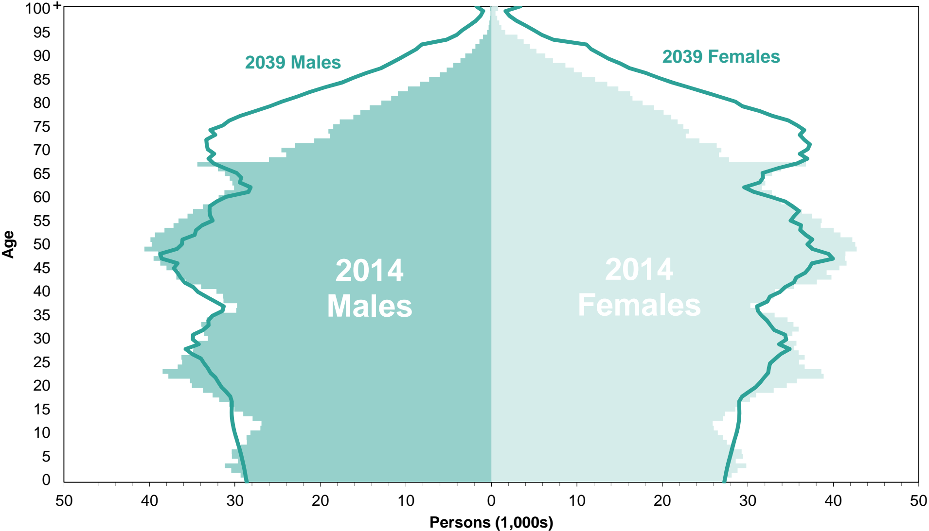
Figure 4: Estimated and projected age structure of the Scottish population, mid-2014 and mid-2039
