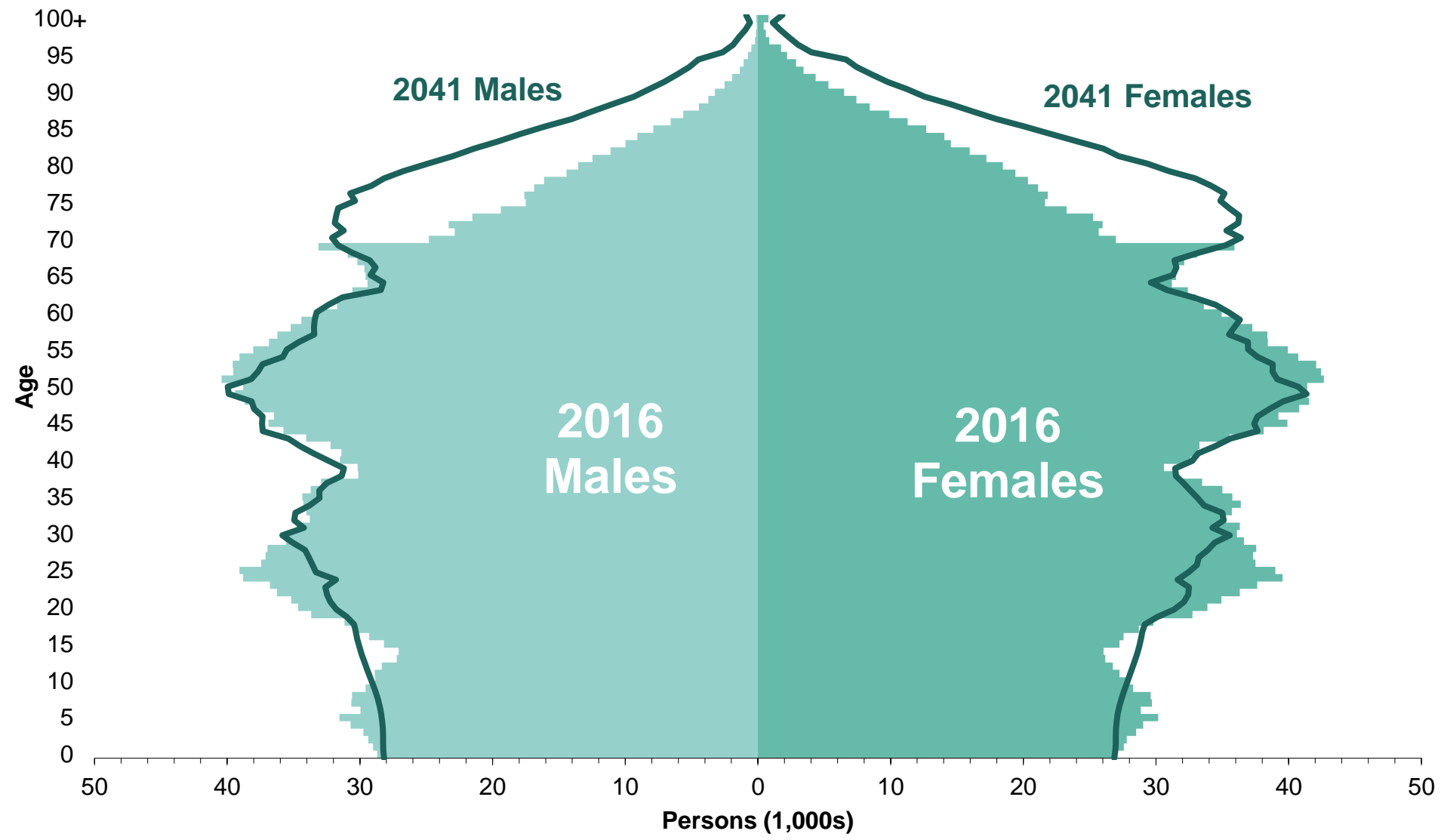
Figure 6: Estimated and projected age structure of the Scottish population, mid-2016 and mid-2041
