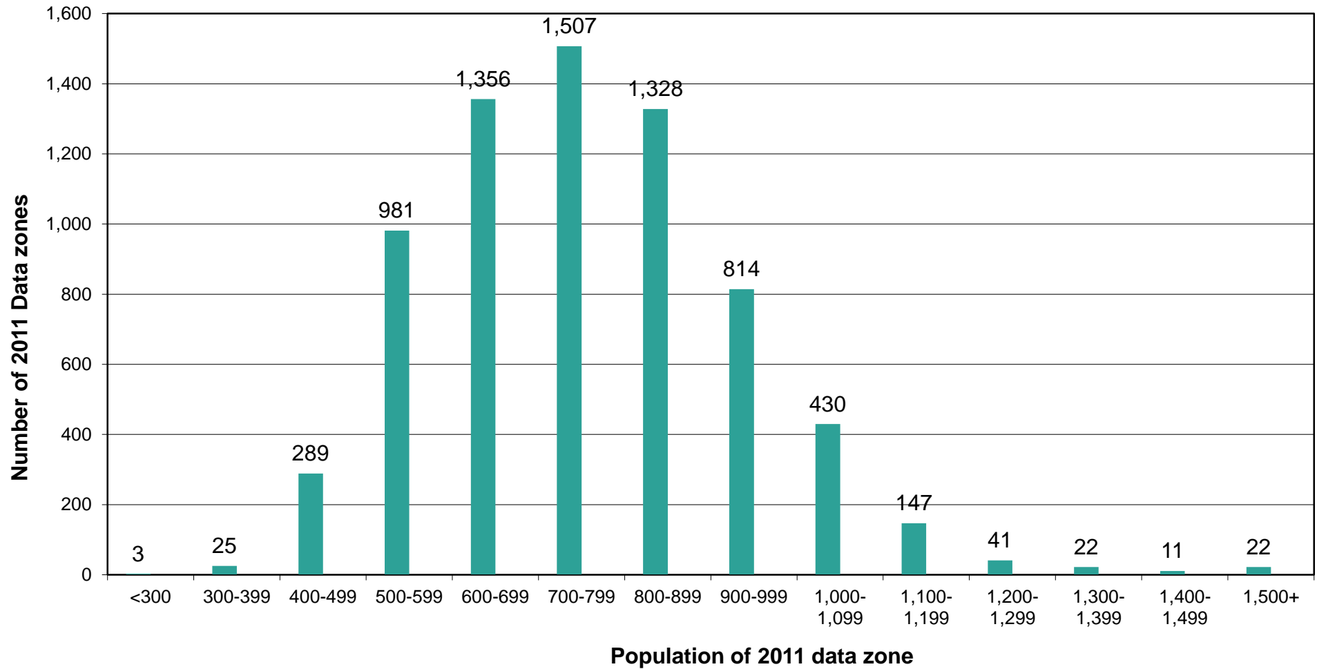
Figure 2.1: Distribution of 2011 Data Zone population, 2014
